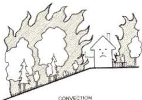
CONVECTION
