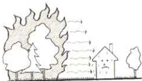
RADIATION
